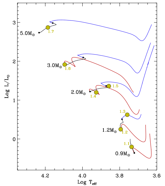
Figure 1. HR diagram showing the targets for Task 1 (see Table 1). Red lines correspond to the PMS, black lines to the MS and blue lines to the post MS evolution (CoRoT reference grid from CESAM). The targets are ordered in mass and age along the diagram, from Case 1.1 (bottom right) up to Case 1.7 (top left).
